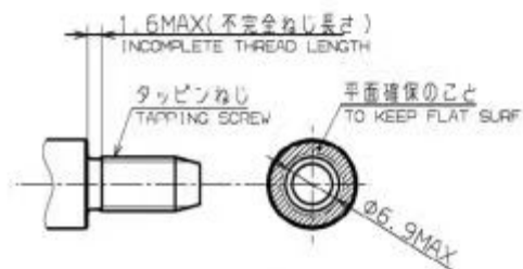
DETAIL AREA D(2:1)
