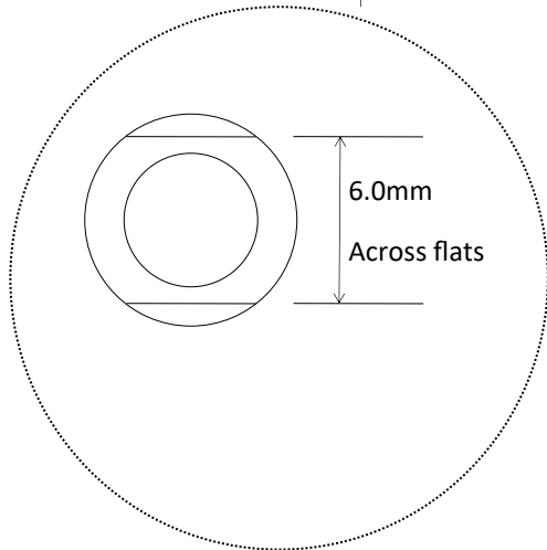
View on A Blown up of rod end for clarity
